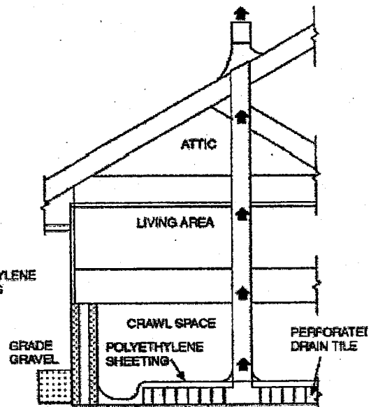
SUBMEMBRANE DEPRESSURIZATION SYSTEM FOR CRAWL SPACE
